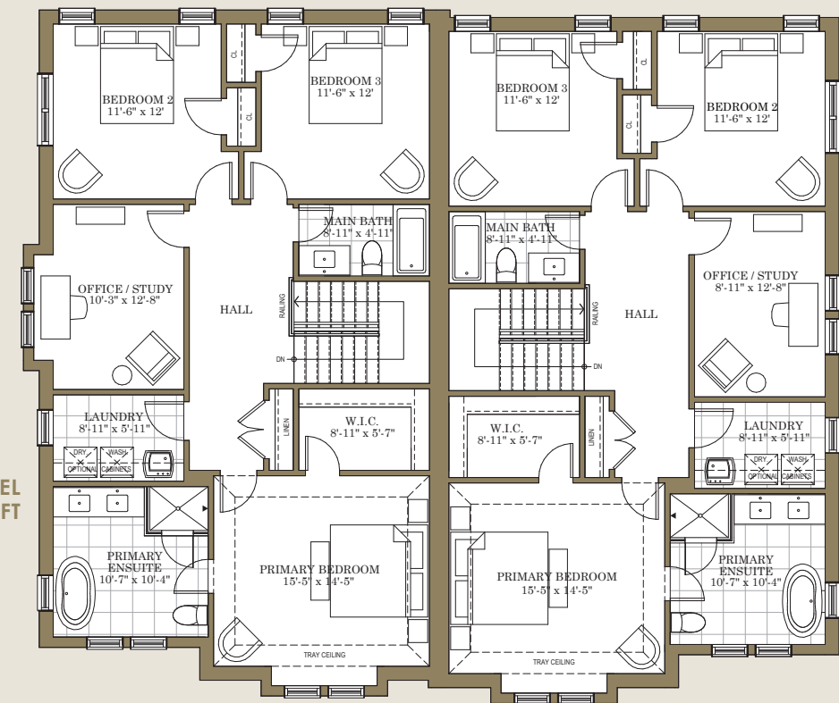
UPPER LEVEL 1244 SQ FT
